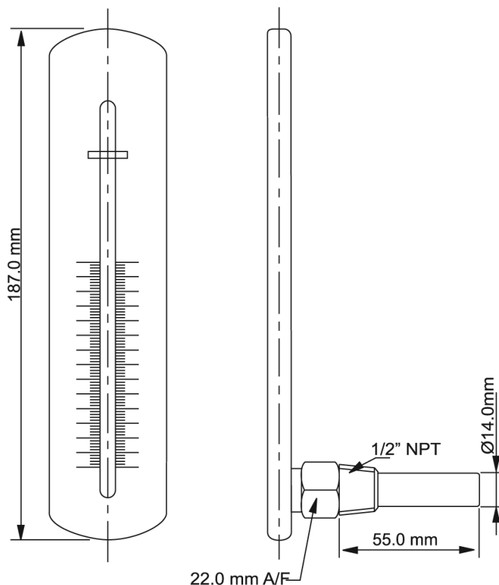
Dimensions - back entry
