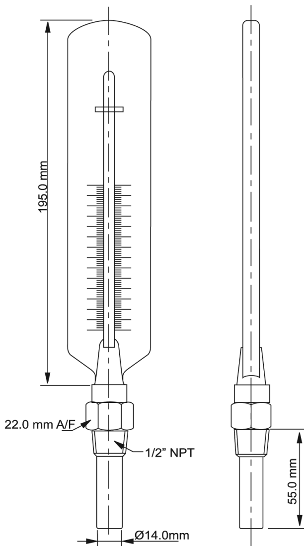
Dimensions - bottom entry
